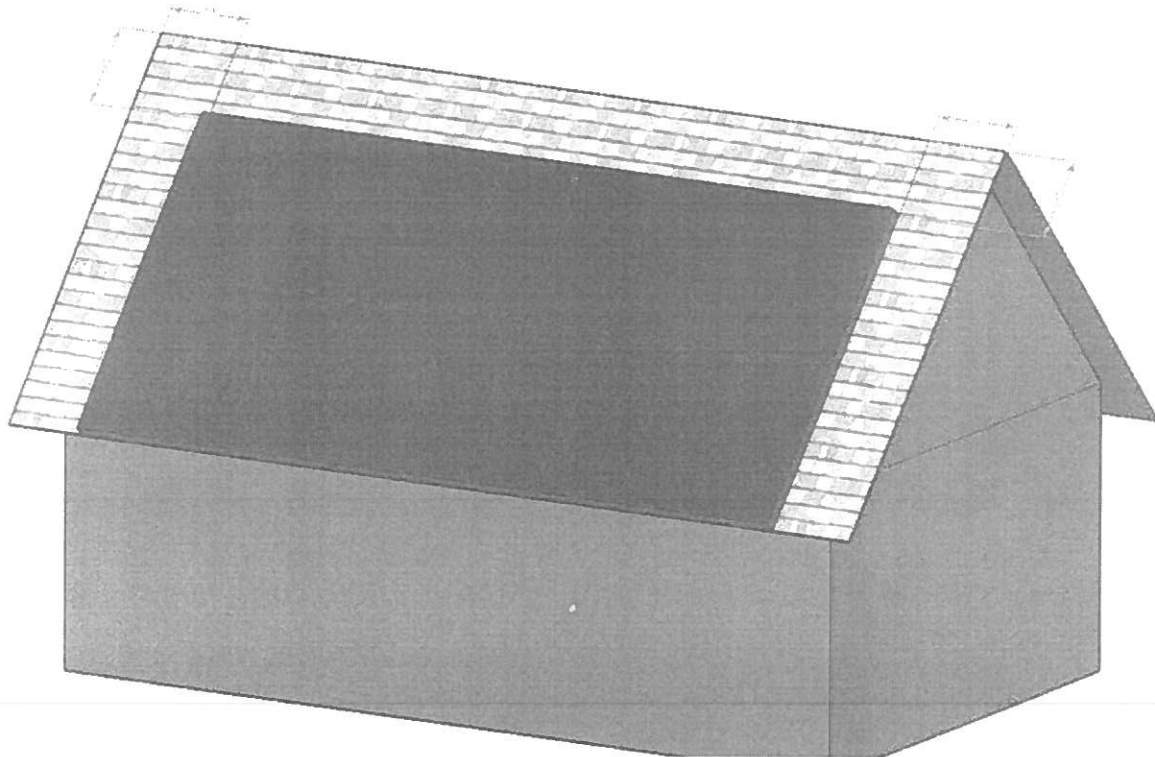
Figure 2 – Single Ridge (IFC 605.11.3.2.2)
